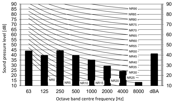
Cooling mode
