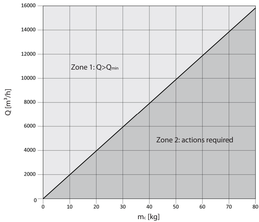
Figure 2: minimum circulation airflow
