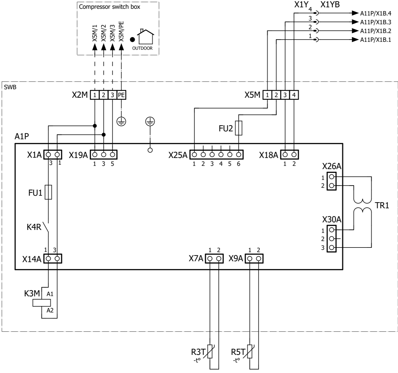
SWB - Control circuit
