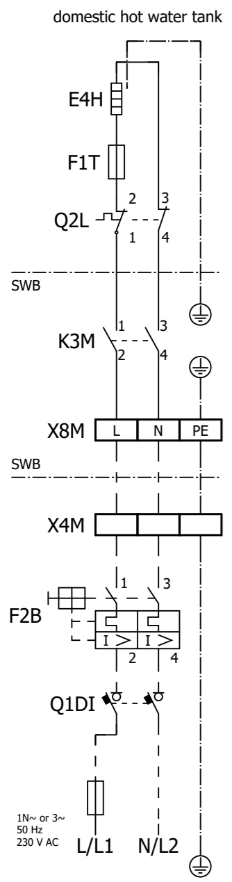
SWB - BSH power supply
