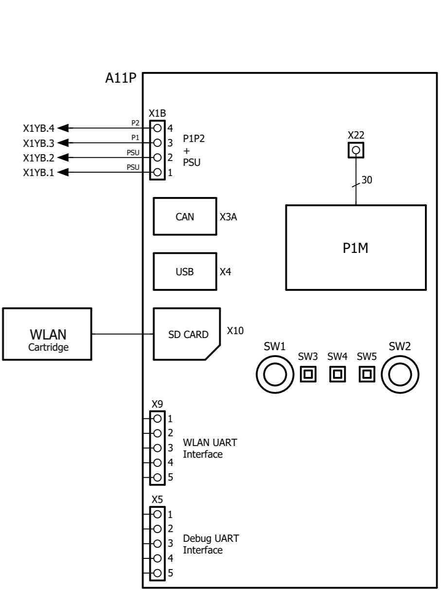
Remote MMI - Control Circuit
