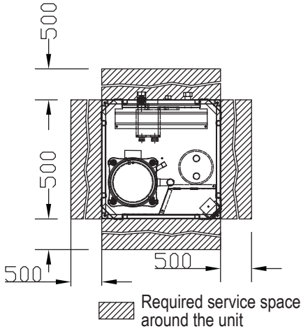
View A-A only for EWLQ 14
