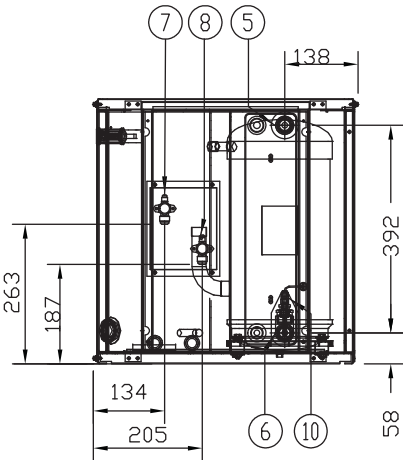
View A-A only for EWLQ 14
