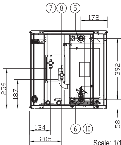
View A-A only for EWLQ 25/33
