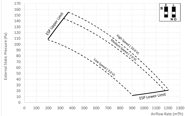
DIP SW (11)
