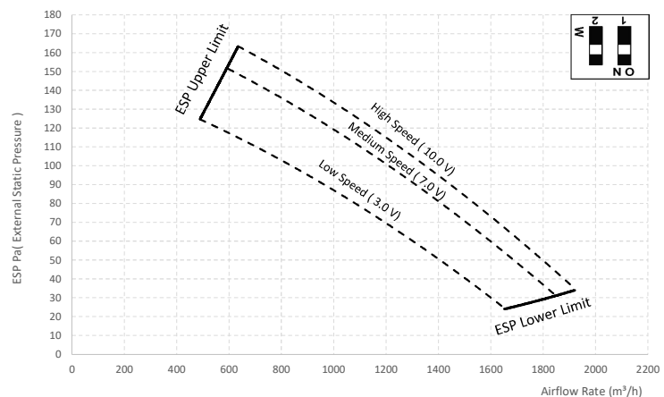
DIP SW (11)
