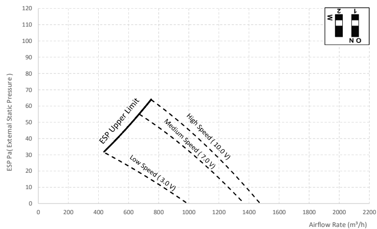
DIP SW (10)
