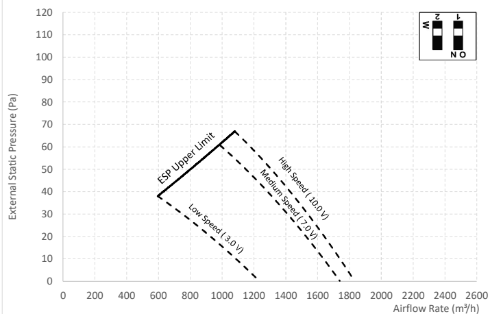
DIP SW (10)
