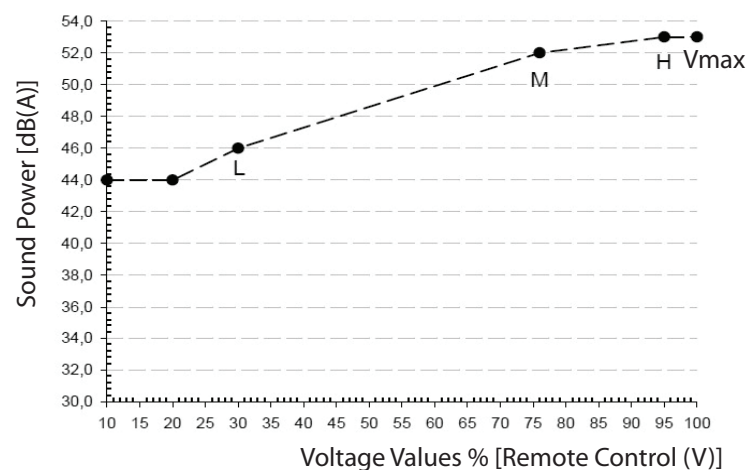
FWQ11AAT Discharge Sound Power
