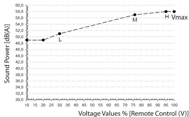
FWQ11AAT Whole Sound Power
