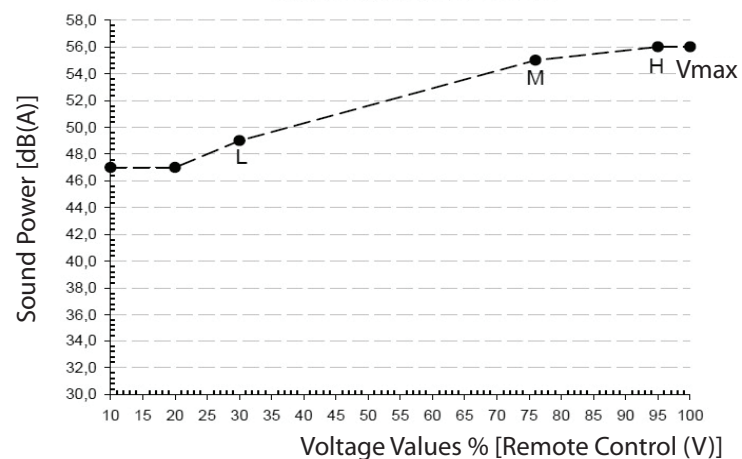
FWQ11AAT Suction Sound Power
