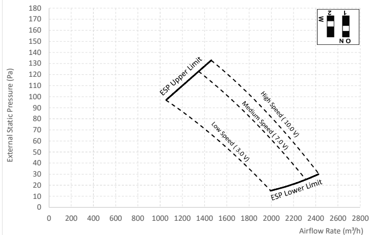
DIP SW (10)
