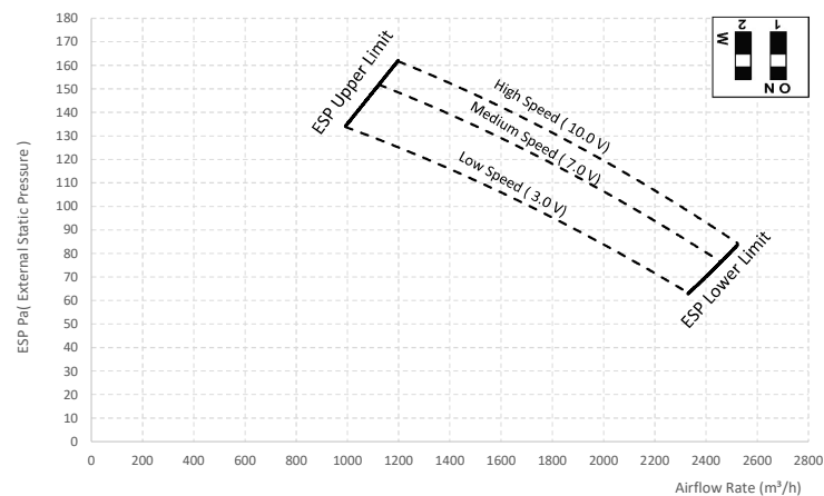
DIP SW (11)
