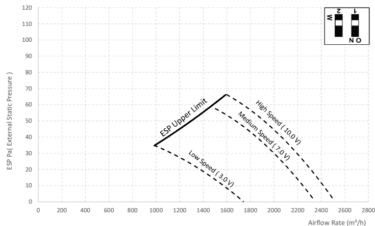
DIP SW (10)
