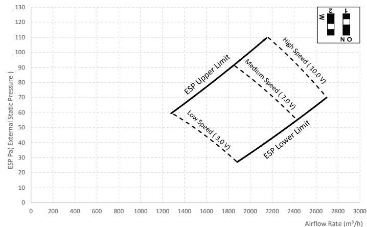
DIP SW (11)
