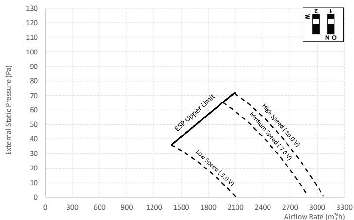
DIP SW (10)
