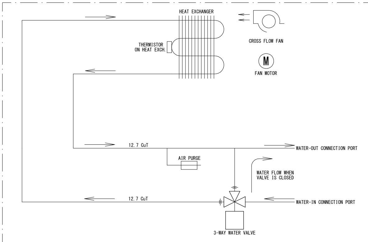
WATER PIPE CONNECTION PORT DIAMETERS
