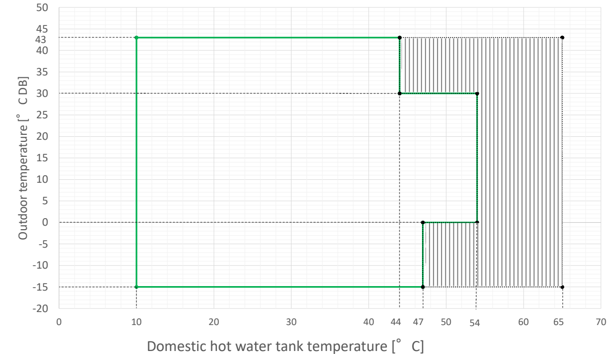
5XXM + CHVX Domestic hot water heating mode
