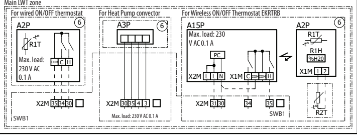
(4) External On/OFF thermostats and heat pump connector
