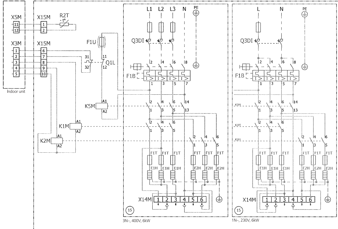
Connection diagram
