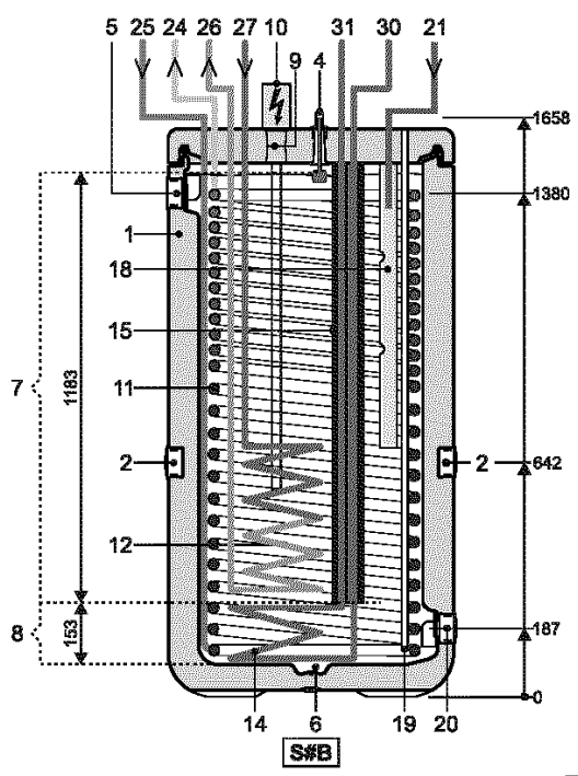
Connections and dimensions, high performance hot water storage tank with solar support.
