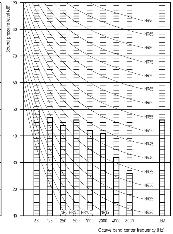
E(D/B)(H/L)Q016* COOLING
