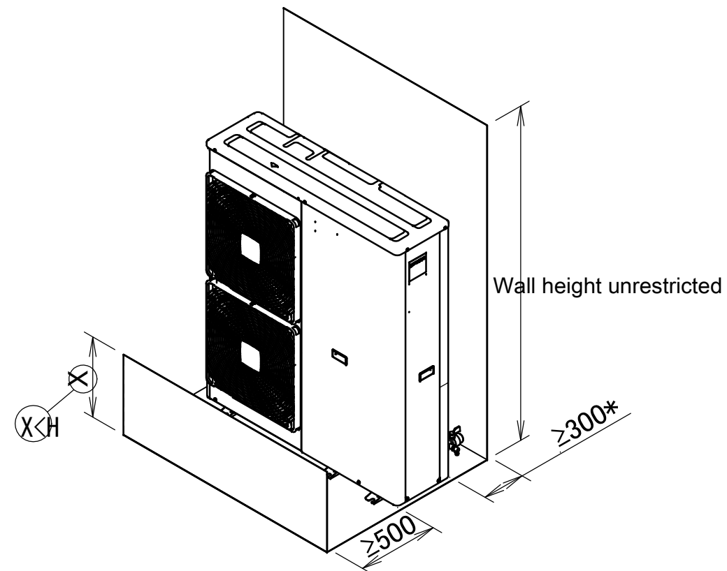
Discharge-side obstacle
