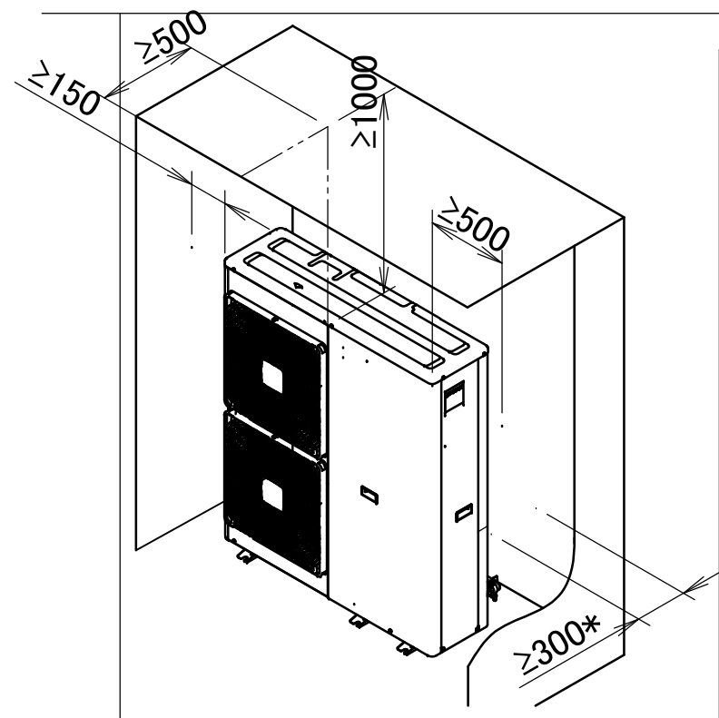
Top-side obstacle
