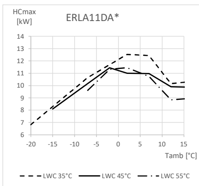
Maximum heating capacity - peak values
