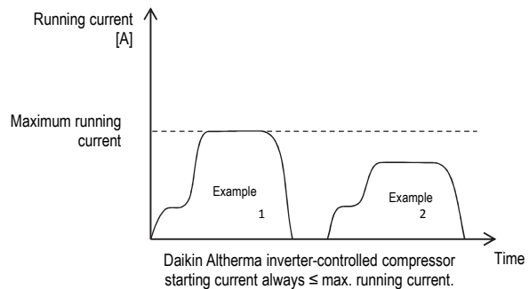
Figure ·A· Starting current
