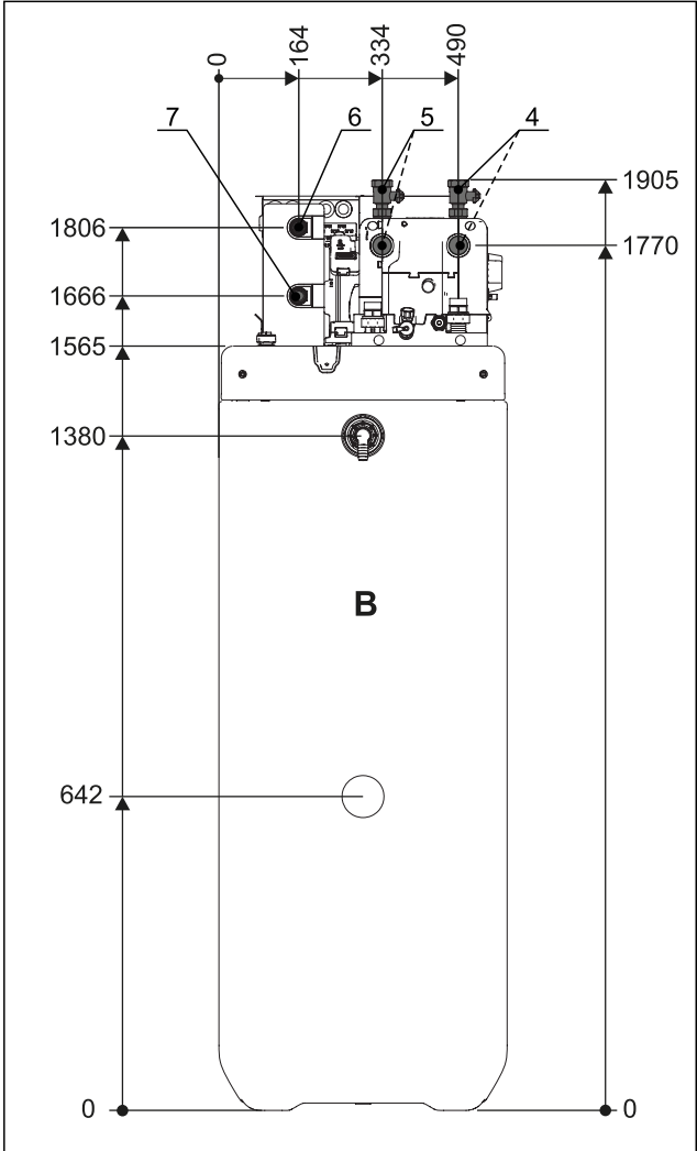
Dimensions, side view – ETS(X/H)B16P30D
