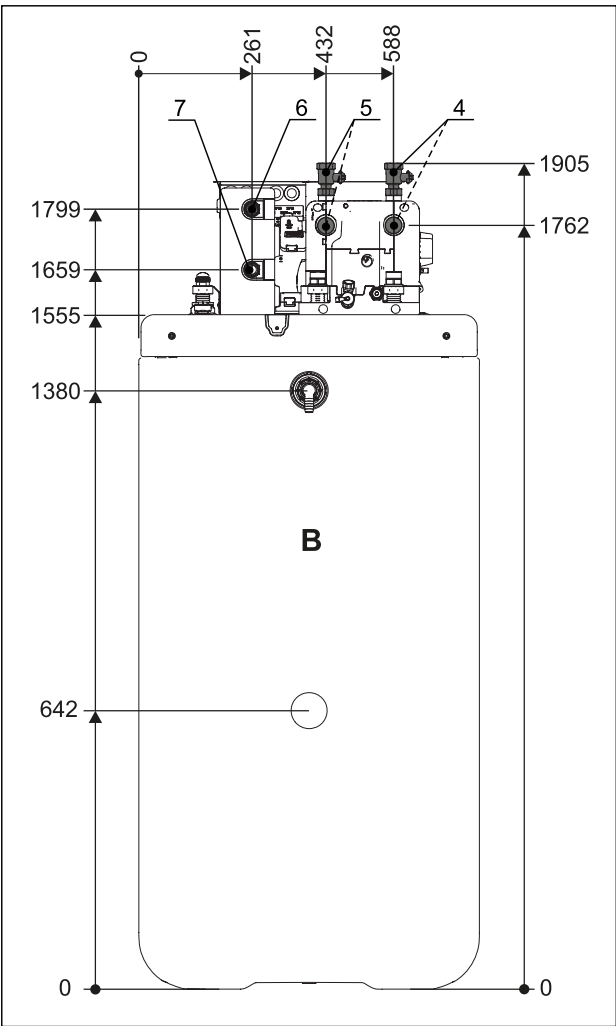
Dimensions, side view – type ETS(X/H)B16P50D
