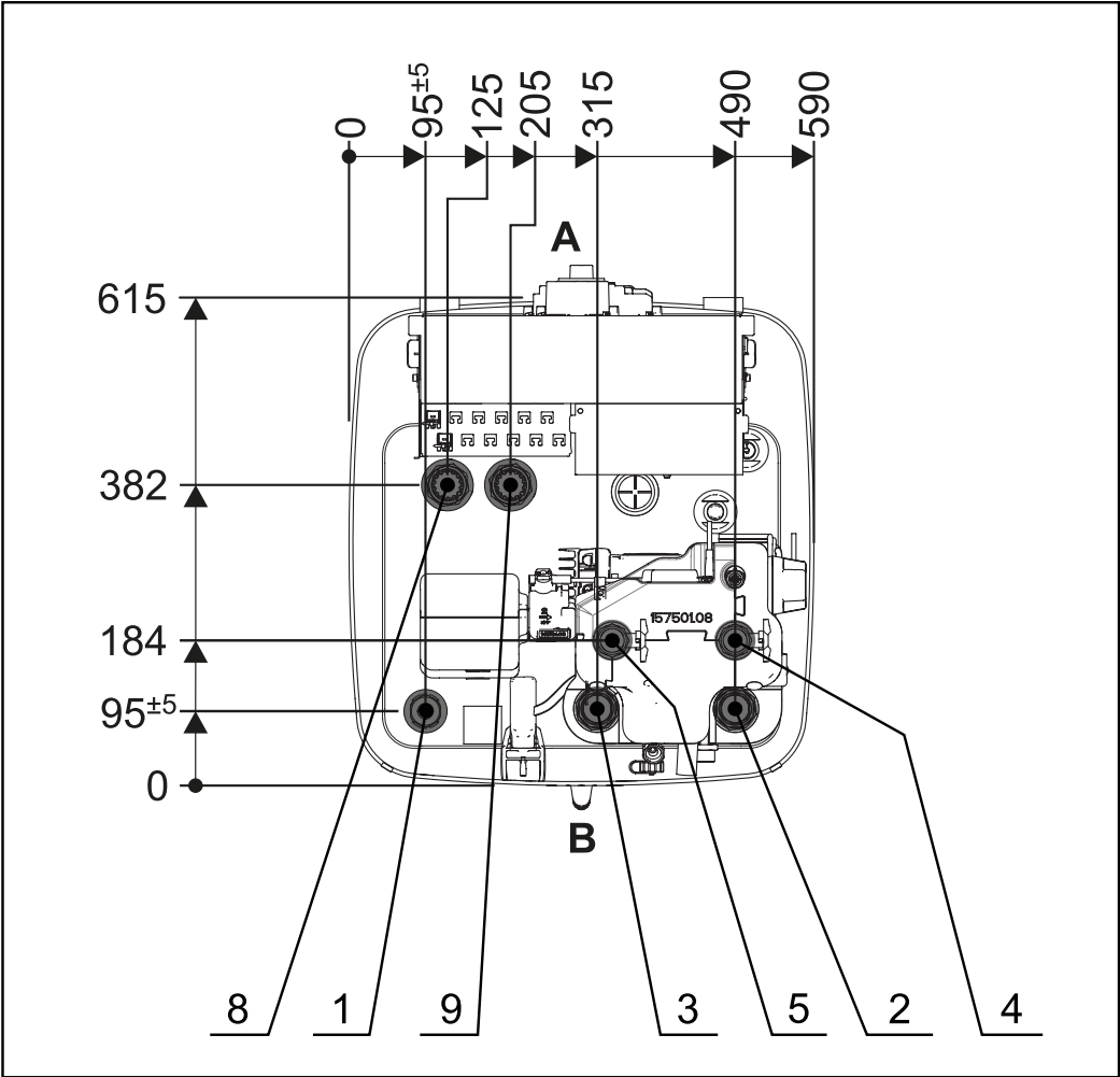
Dimensions, top of unit – type ETS(X/H)B16P30D
