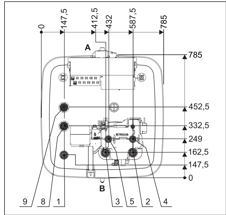
Dimensions, top of unit – type ETS(X/H)B16P50D
