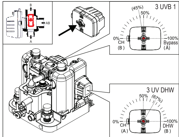
Function 3-way diverter valve
