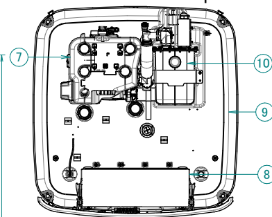
top view without hood
