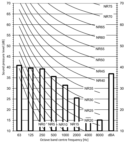
EPSK06ARV3
