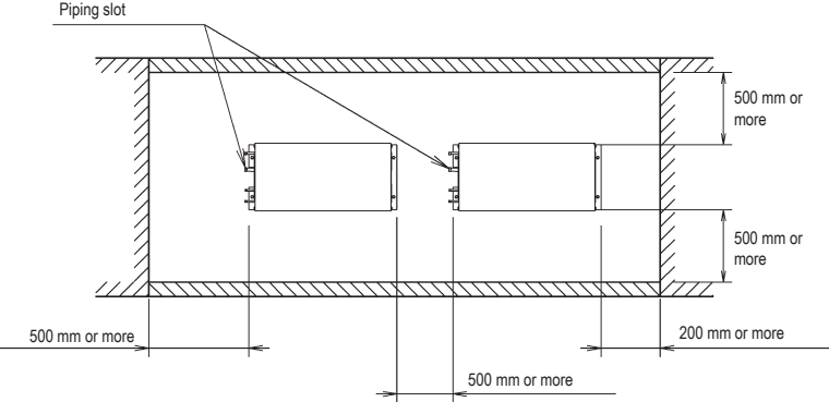
When installed in serial
