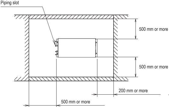
When installed as a single unit
