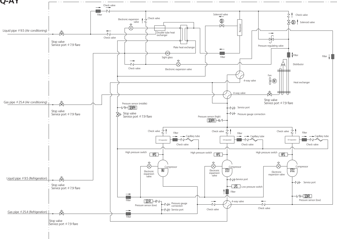
Outdoor unit
