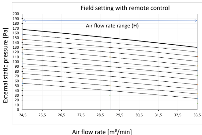
Fan characteristics (2)
