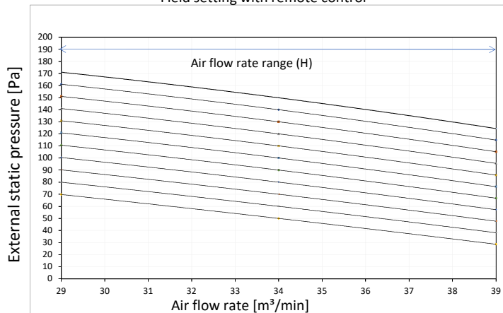
Fan characteristics (2)
