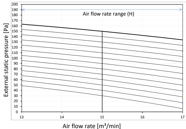
Fan characteristics (2)
