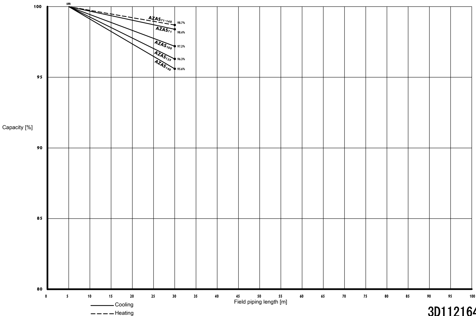
Capacity in function of field piping length
