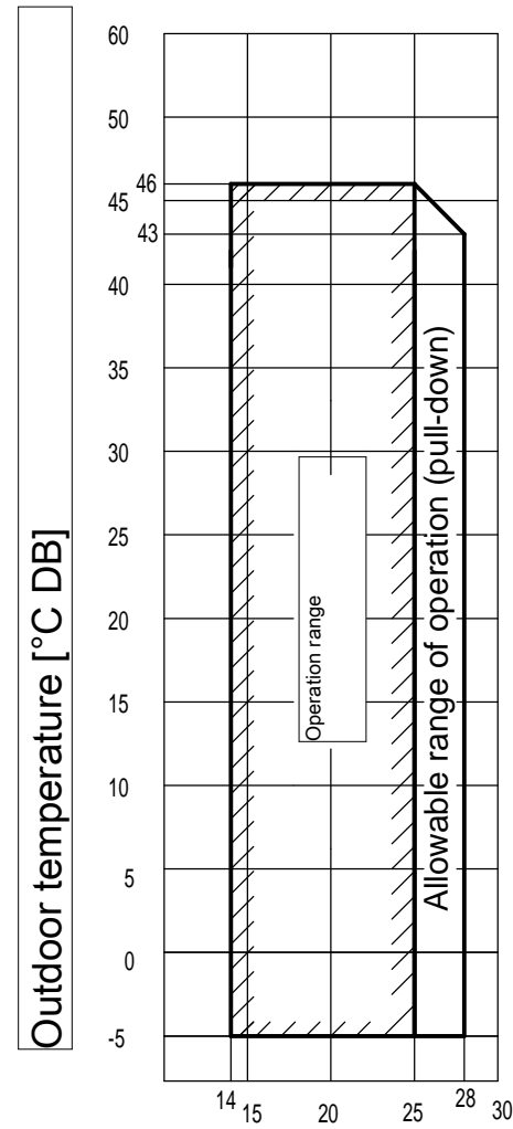
Indoor temperature [°C WB]
