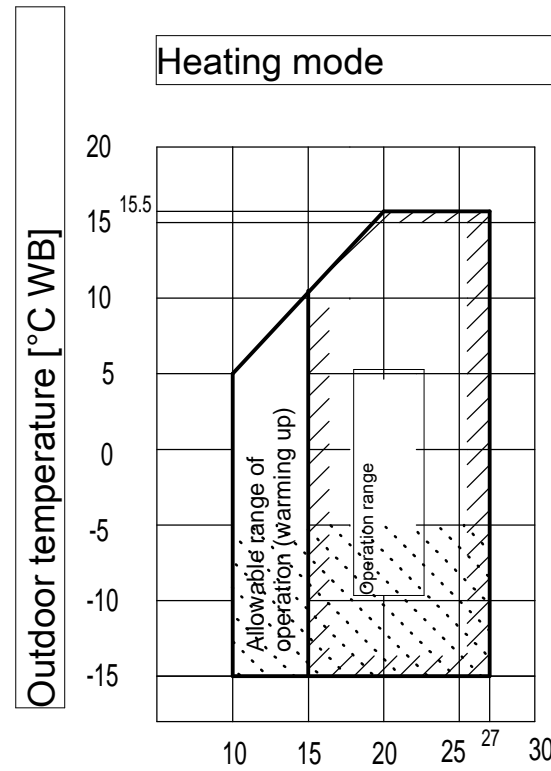
Indoor temperature [°C DB]
