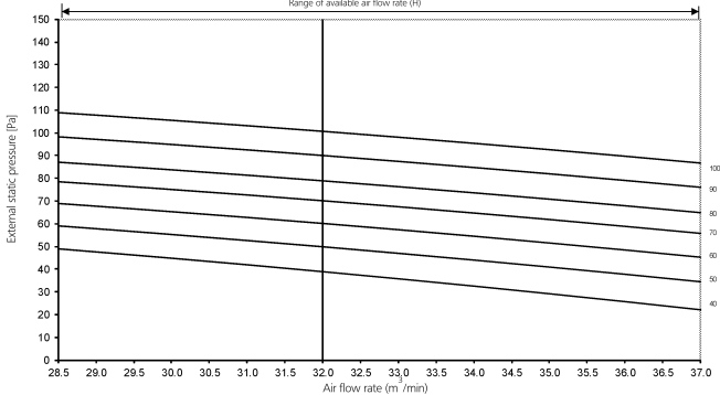
Fan characteristics (2) (Field setting with remote controller)
