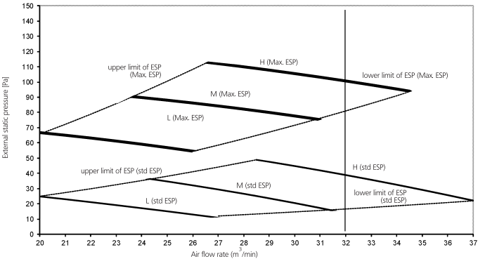
Fan characteristics (2) (Field setting with remote controller)
