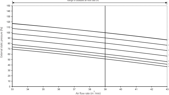
Fan characteristics (2) (Field setting with remote controller)
