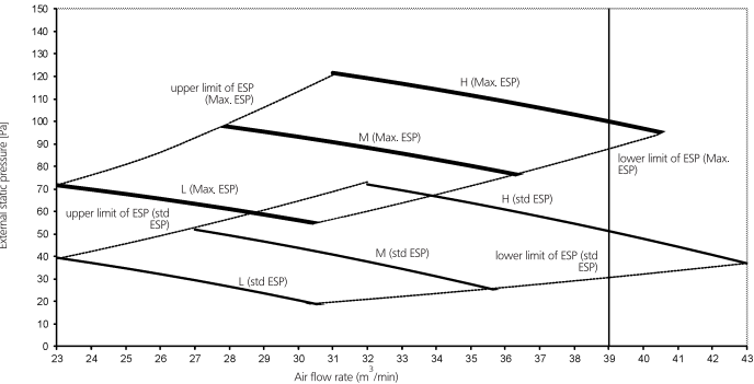
Fan characteristics (2) (Field setting with remote controller)
