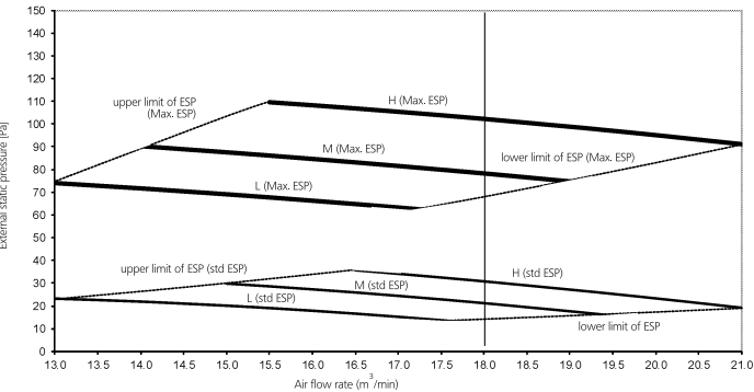
Fan characteristics (2) (Field setting with remote controller)
