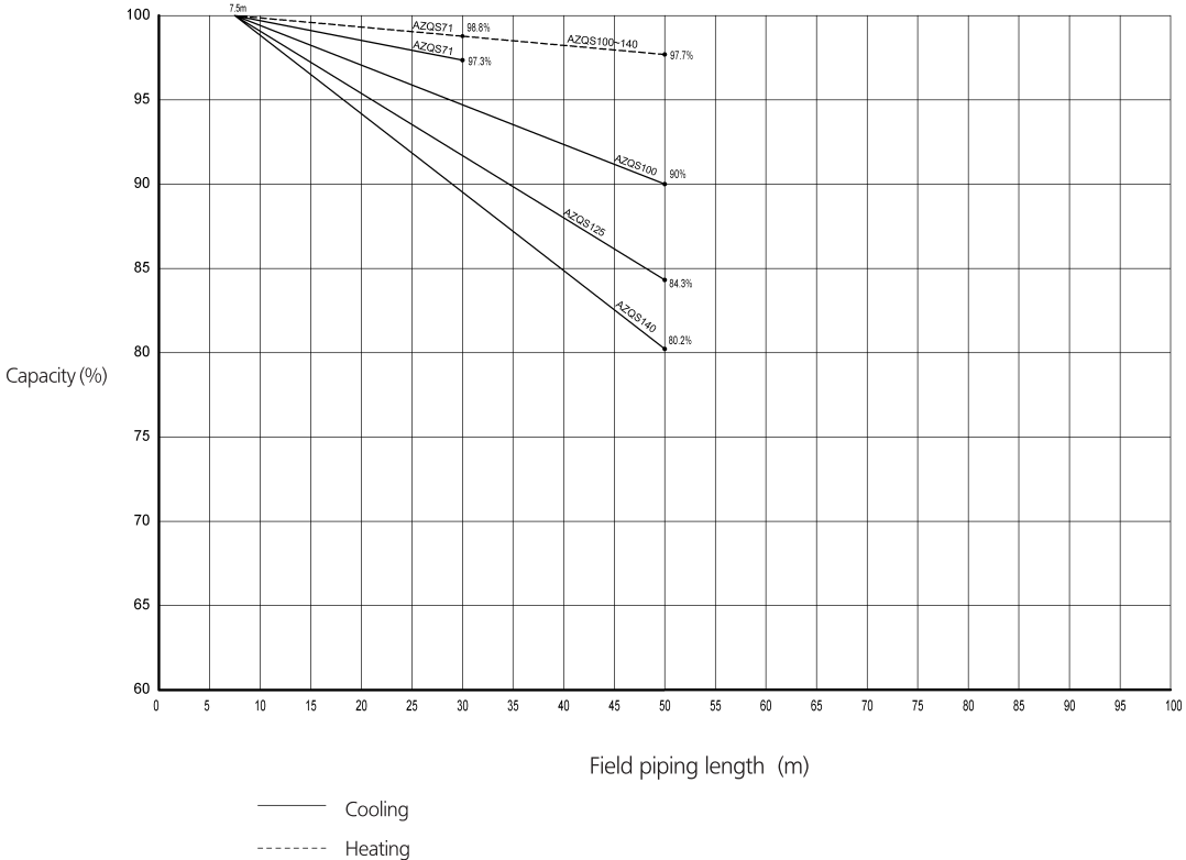
Capacity in function of field piping length for inverter
