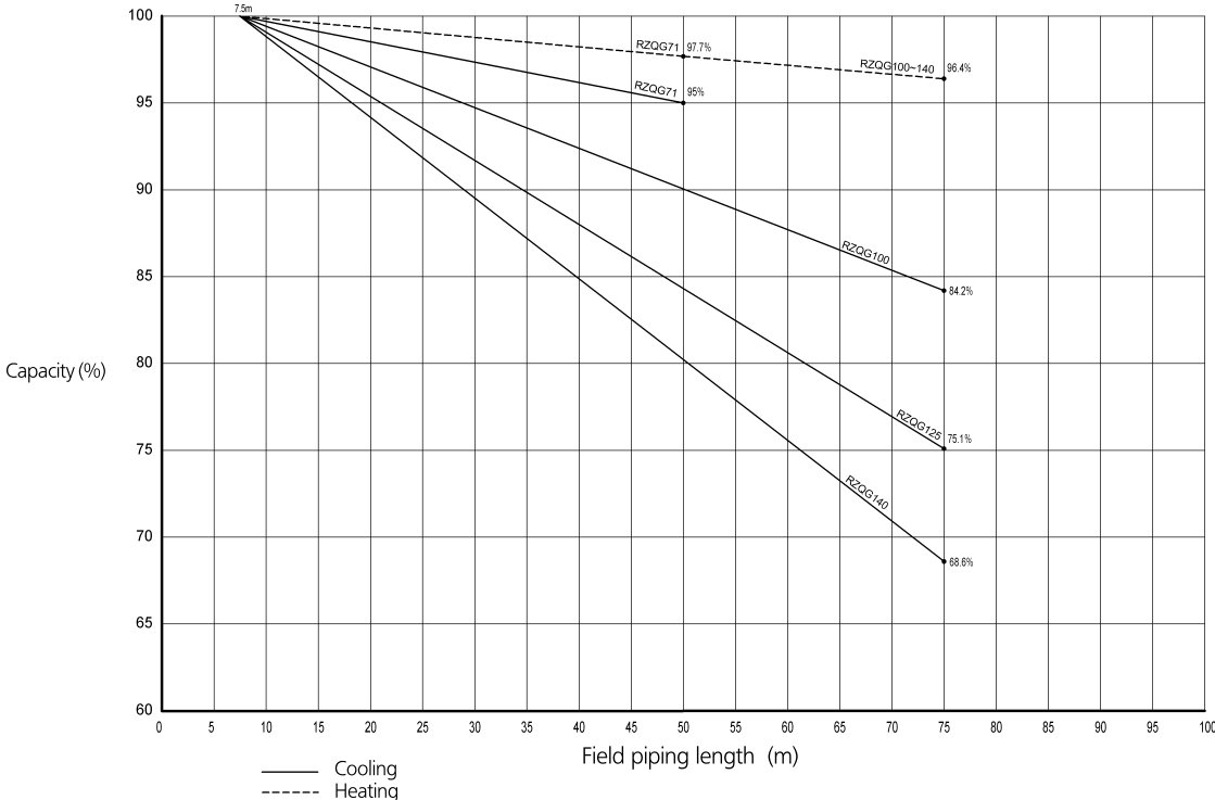
Capacity in function of field piping length for inverter
