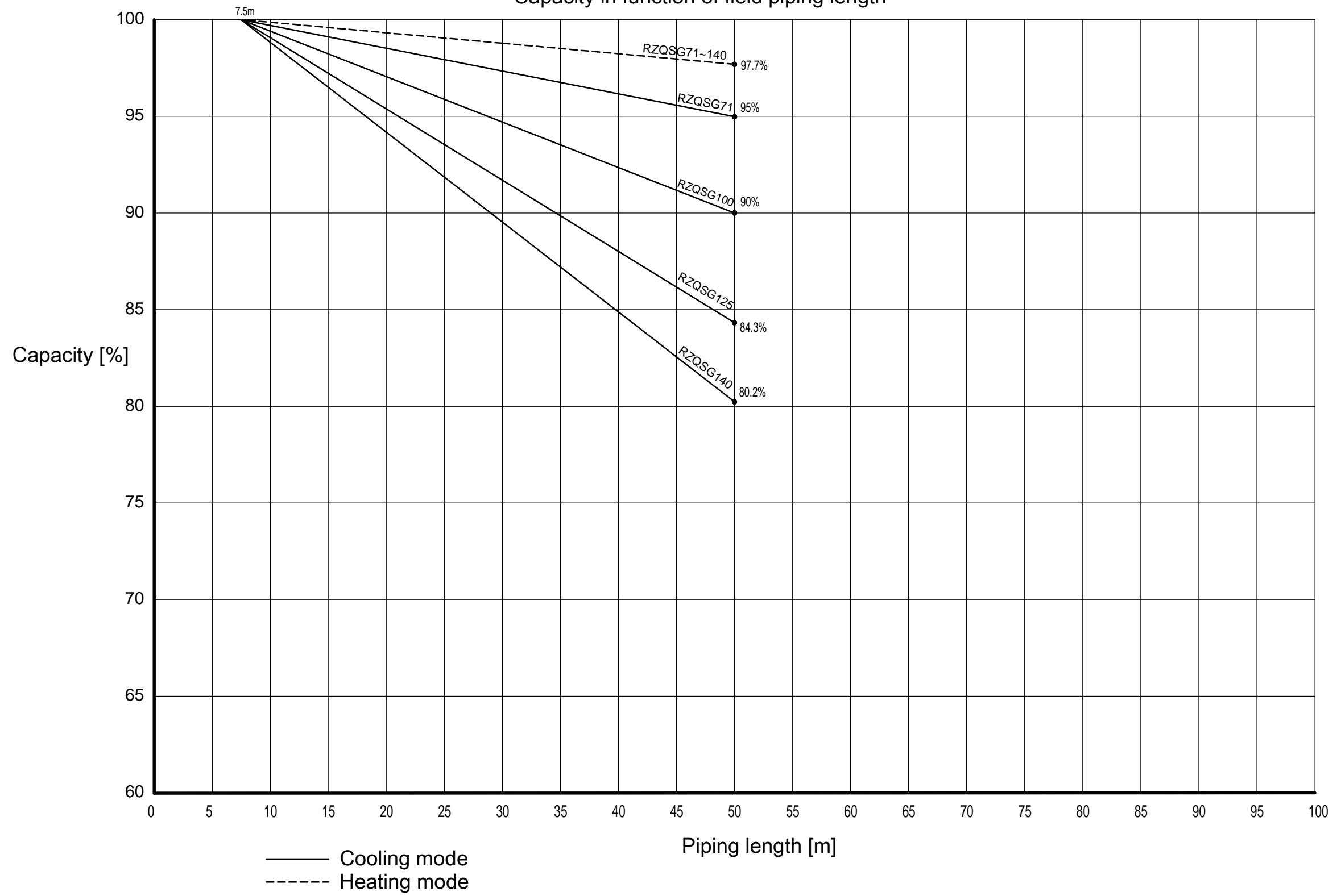
Capacity in function of field piping length
