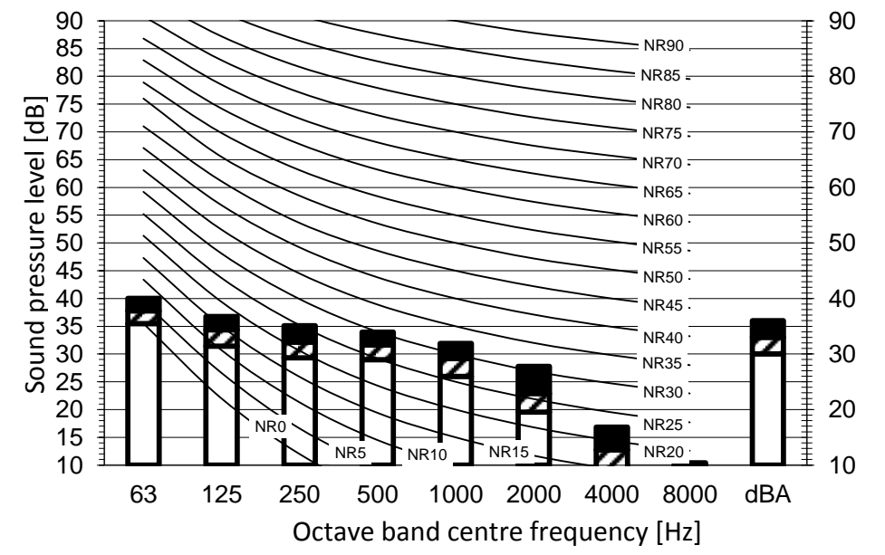
Heating mode
