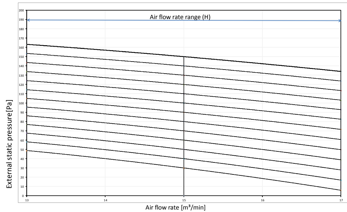
Fan characteristics (2) Field setting with remote control
