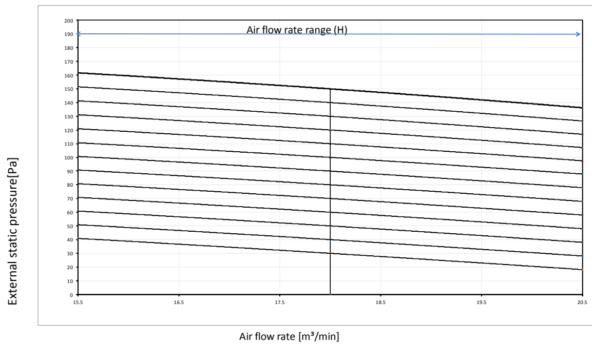
Fan characteristics (2) Field setting with remote control
