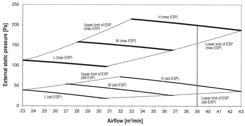
Fan characteristics (1)
