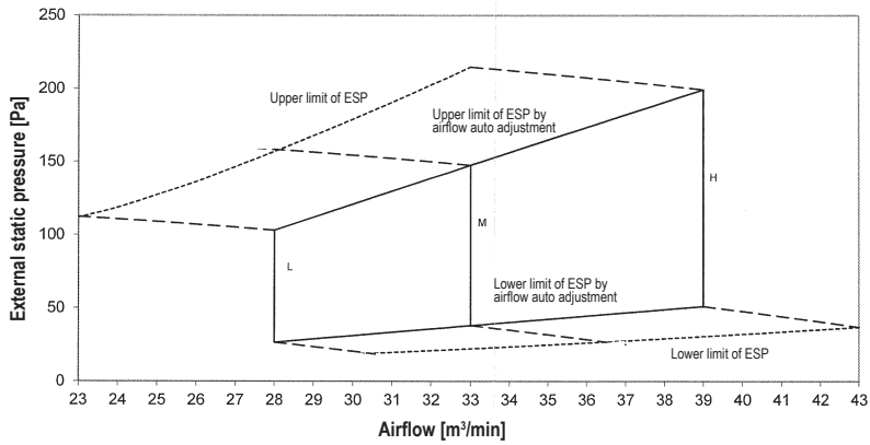
Fan characteristics (3) (airflow auto adjustment)
