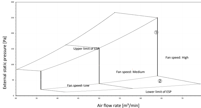
Fan characteristics (3) Air flow auto adjustment
