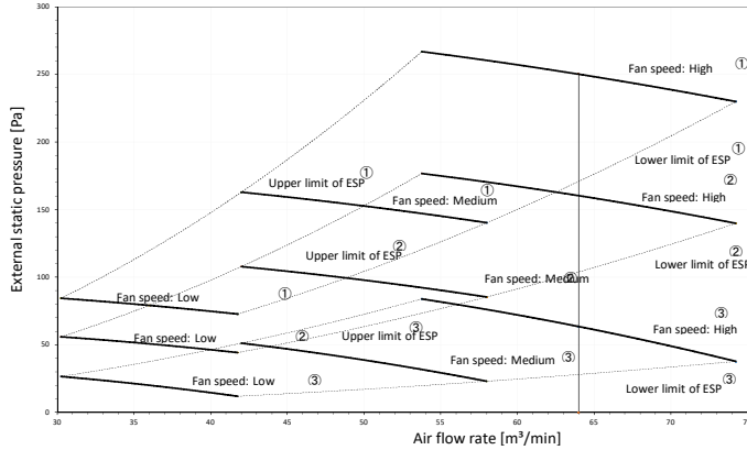
Fan characteristics (3) Air flow auto adjustment
