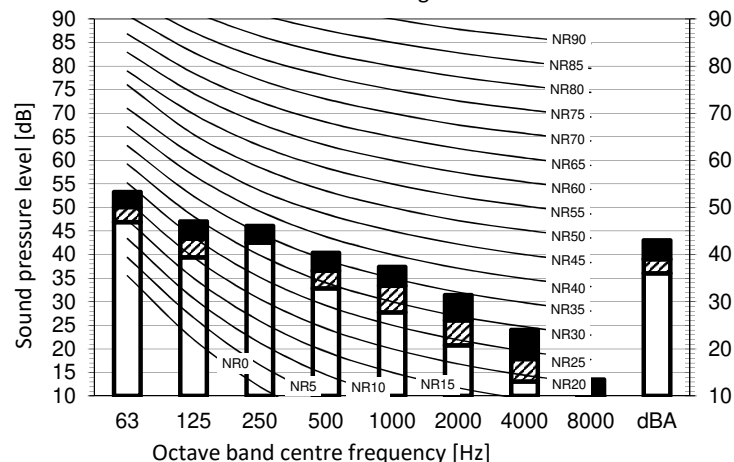
Heating mode
