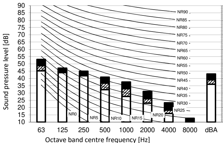
Cooling mode
