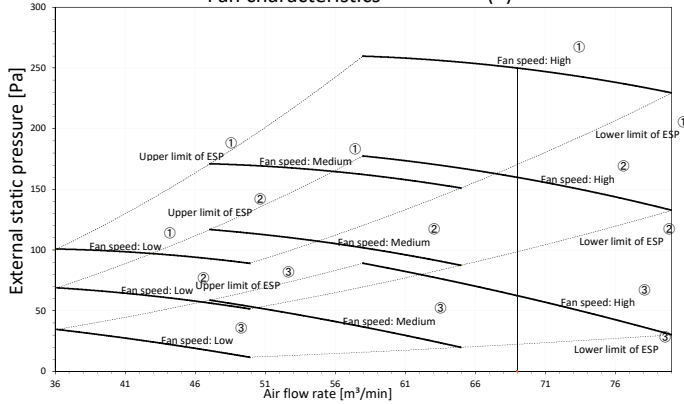
Fan characteristics (3) Air flow auto adjustment
