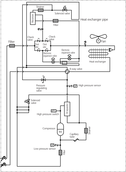
Outdoor unit
